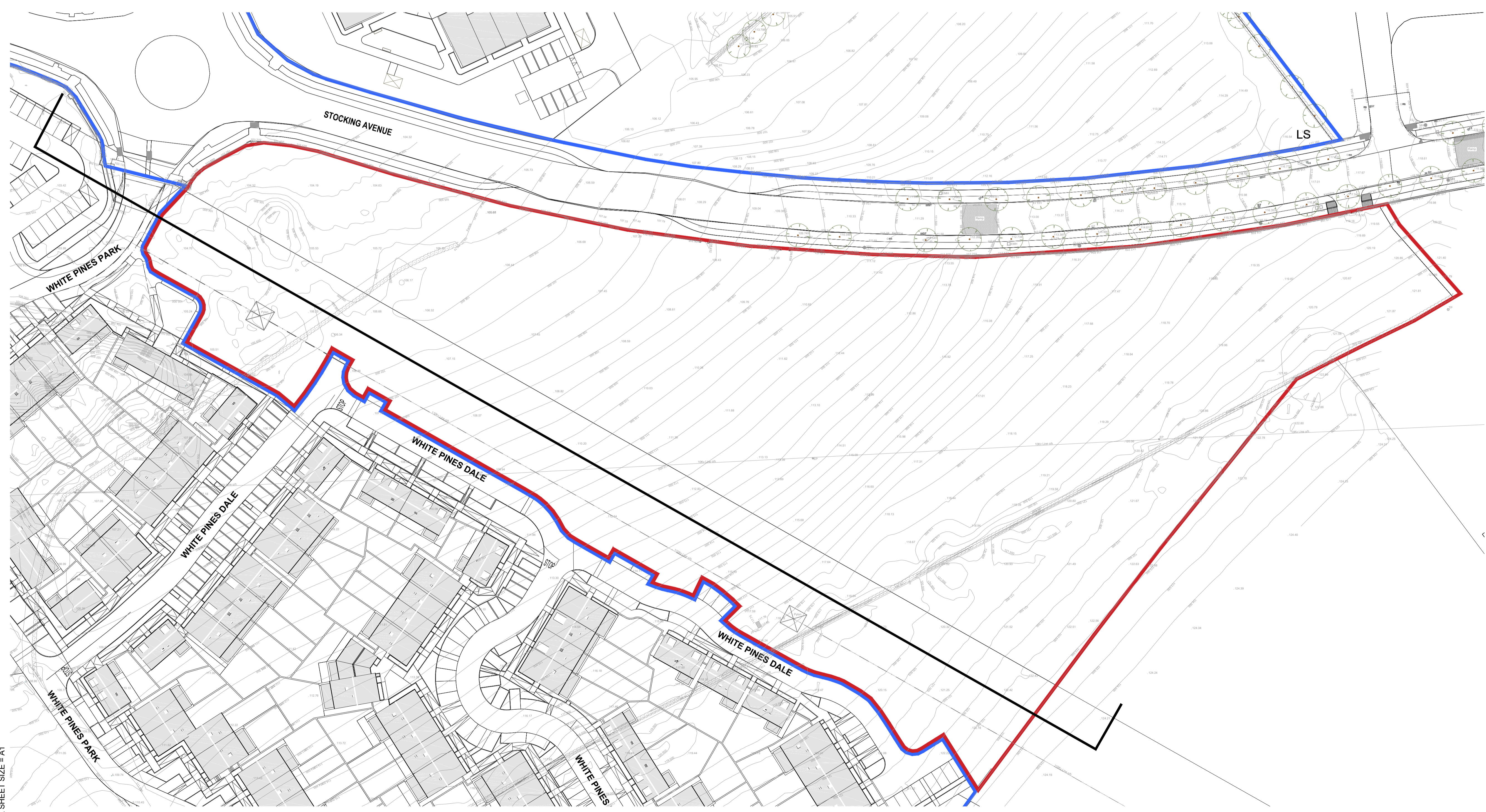
2 TOPOGRAPHICAL SURVEY 1:500
